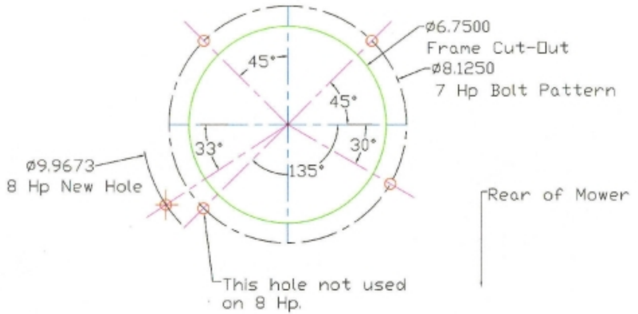
Top View of Frame
